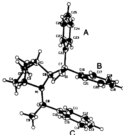
Figure 1. ORTEP drawing of compound 4.
